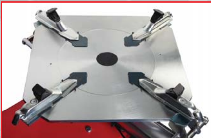
Centre-Clamp design with covered sliding grooves ensure operator safety
